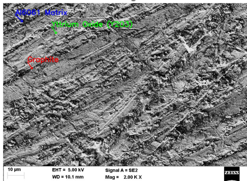
Fig 3: SEM image of hybrid composite
