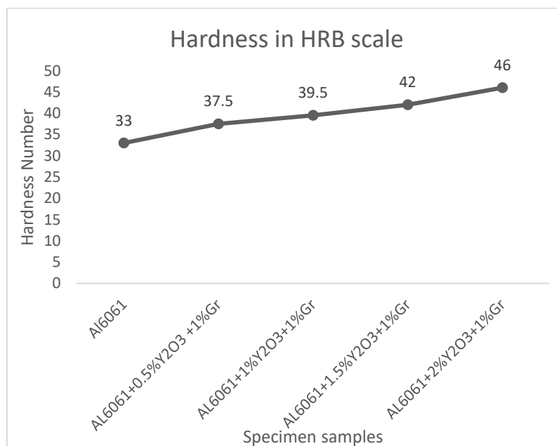
Fig 13: Result of hardness test for all the specimens
