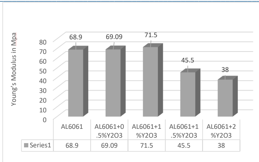
Fig 12: Young's modulus of all the specimens
