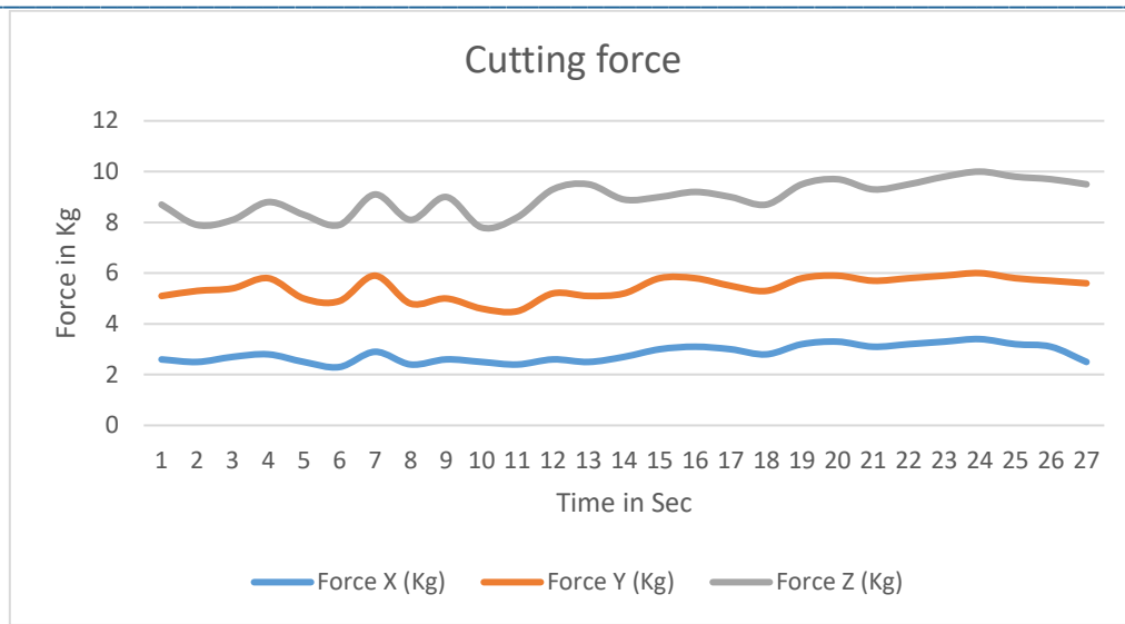
Fig 9: cutting force graph for the specimen 2 (1% Yttrium oxide & 1% Graphite)
