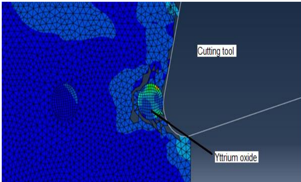
Fig 14: Virtual machining of the model by FEA method using Ansys software.
