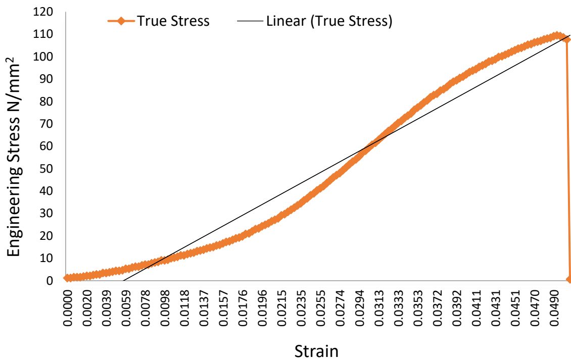
Fig 11: stress strain graph generated from tensometer result.
