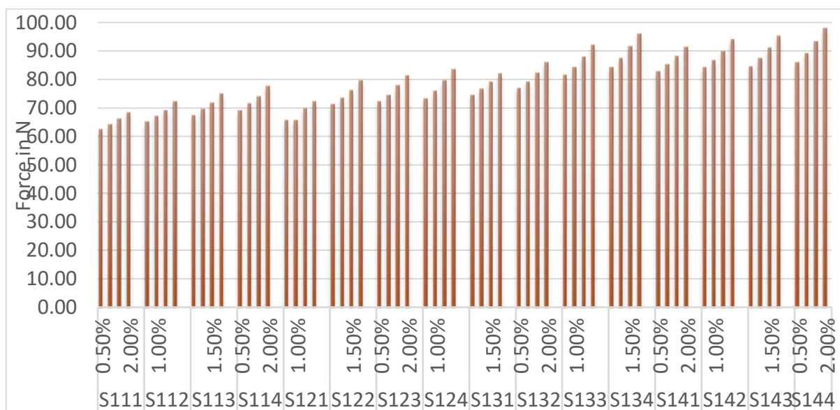
Fig 10: Bar chart for cutting force on all the specimens
