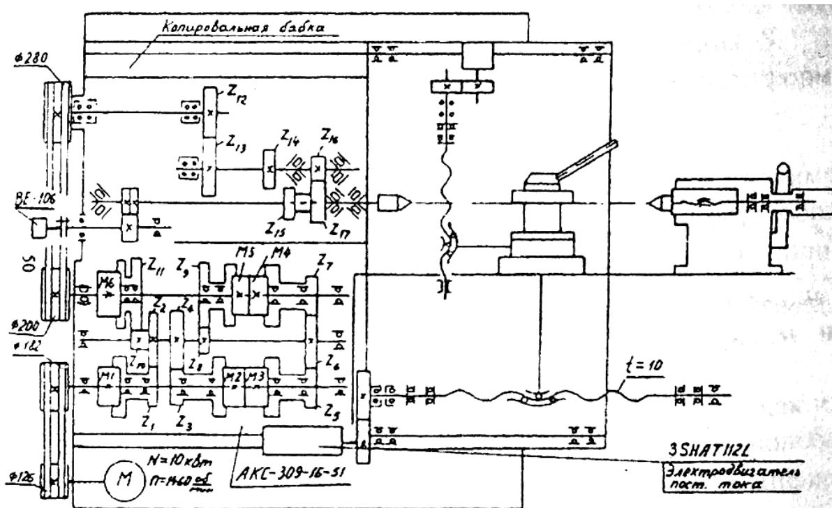
Fig.1. Kinematic diagram of the drive machine with CNC 16K20T1
