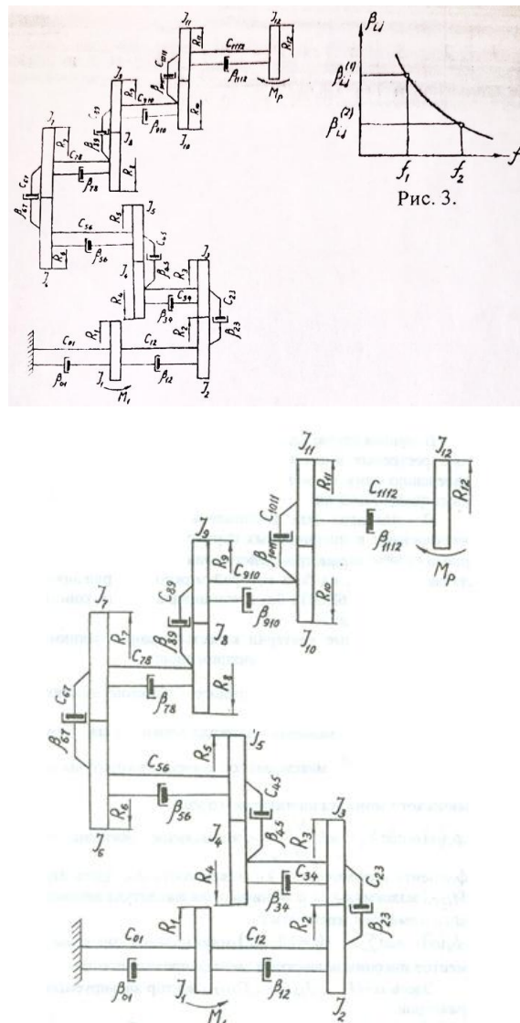
Fig. 2. Dynamic model of the main drive of a CNC lathe 16K20T1 n_{min} = 71 \text{ об/мин}
