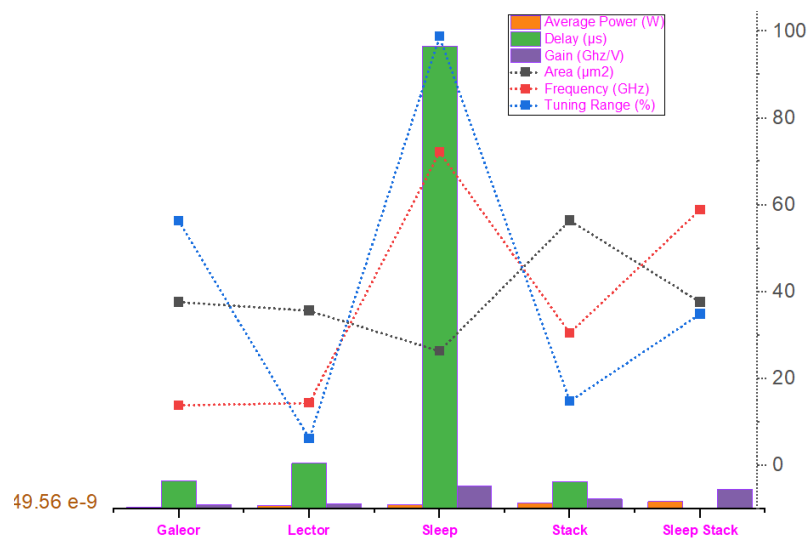
Figure 3. CSVCO parameter analysis using a variety of low leakage power techniques
