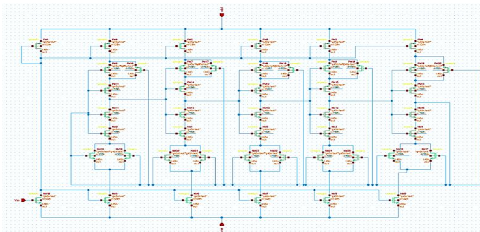
Figure 2. Sleep stack technique for the current starved VCO The Circuit
