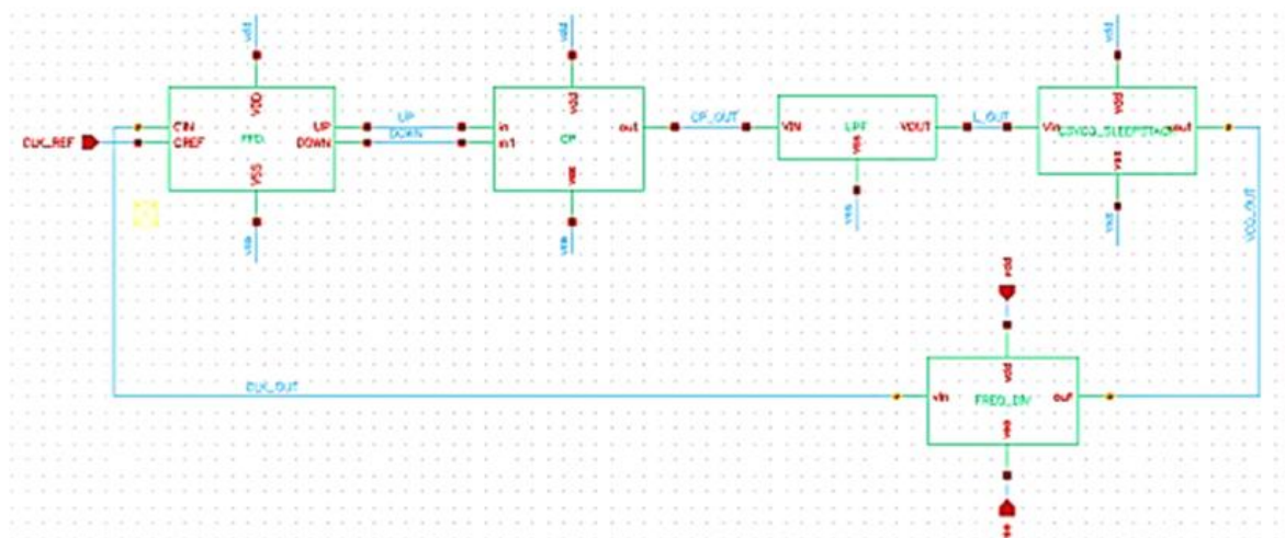
Figure 1. PLL Architecture with Sleep Stack CSVCO
