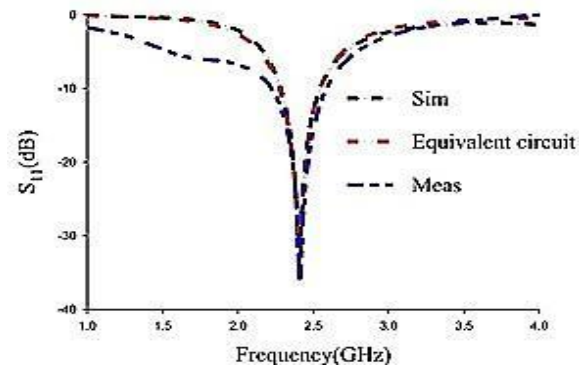
Figure 7. Comparison of the simulated and measured reflection coefficient of the proposed antenna (i.e. Antenna_5)
