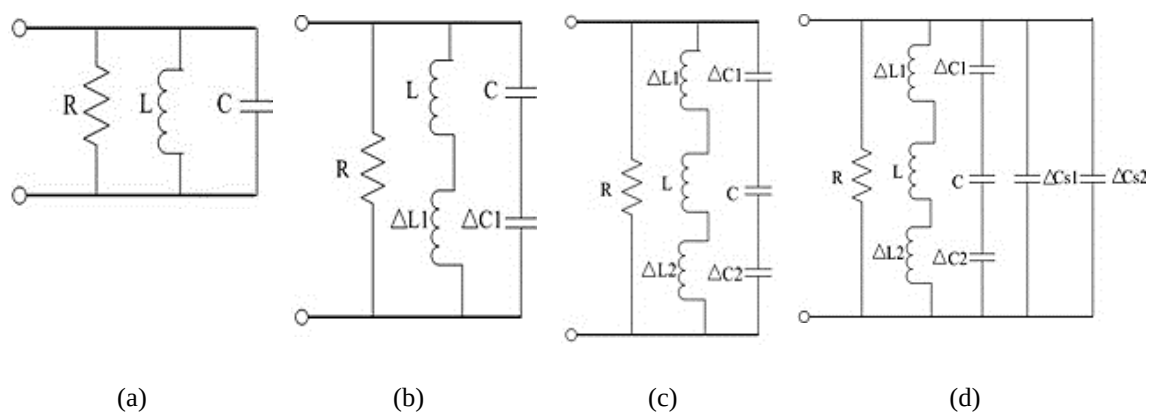
Figure 4 Equivalent circuits of the evolutionary phases of the proposed antenna. (a) Antenna_1 (b) Antenna_2 (c) Antenna_4 (d) Antenna_5
