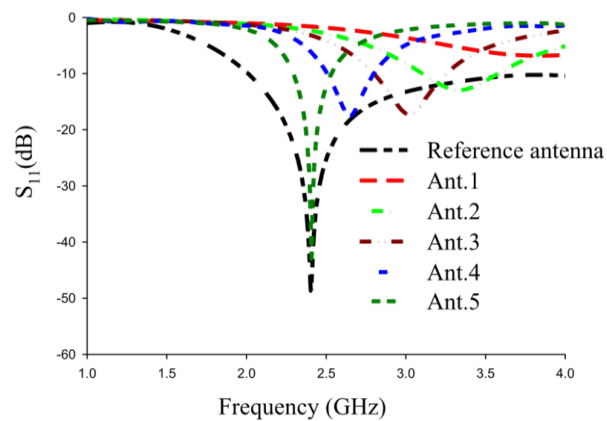
Figure 5. Simulated reflection coefficients at various antenna configurations
