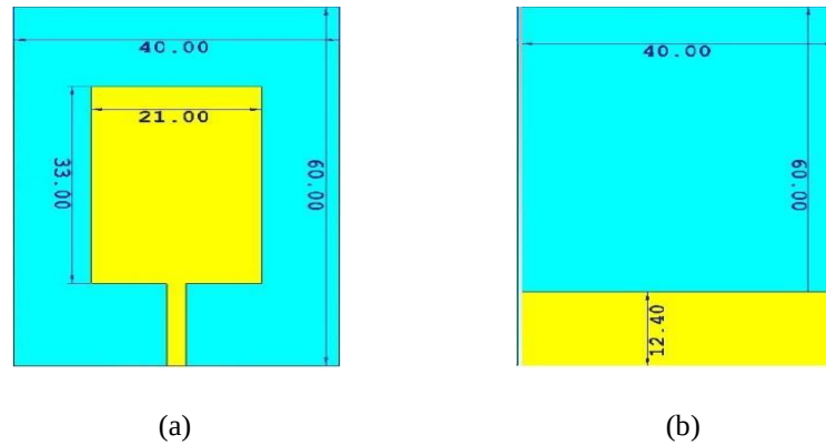
Figure 1. Reference rectangular patch antenna (a) front view, (b) back view.
