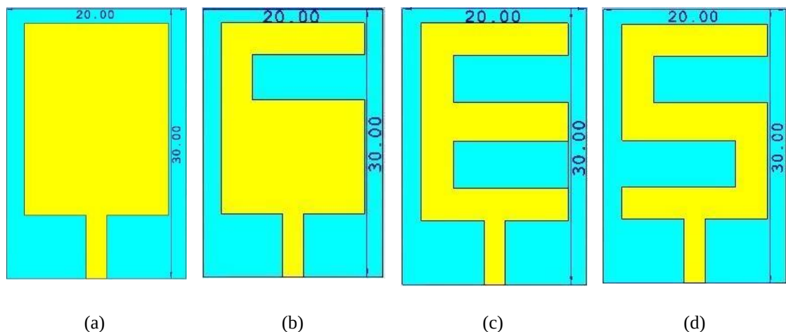
Figure 2. Evolutionary phases of the proposed antenna (a) Antenna_1 (b) Antenna_2 (c) Antenna_3 (d) Antenna_4
