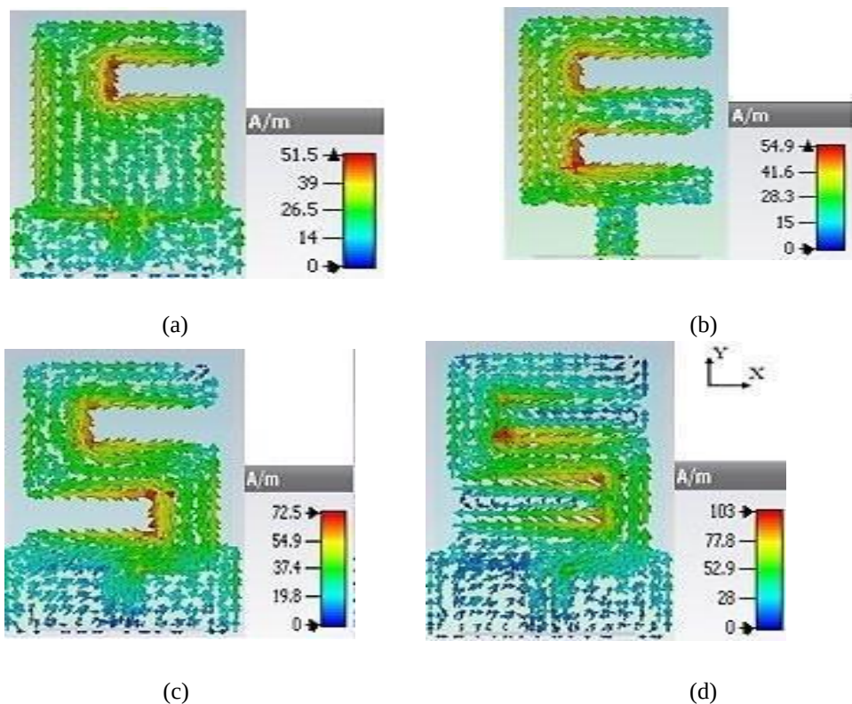
Figure 6. Simulated surface current distribution of the antenna at various frequencies. (a) Antenna_3 (3.334 GHz), (b) Antenna_4 (3.022 GHz), (c) Antenna_5 (2.65 GHz) (d) Antenna_6 (2.4 GHz)
