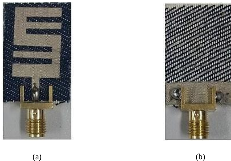
Figure 8. Prototype of the proposed antenna (a) Front view (b) Back view
