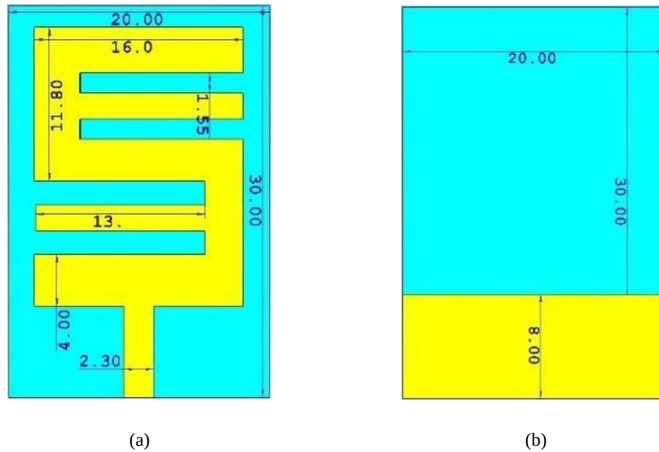
Figure 3. (a) Front view (b) Back view of the proposed antenna (Antenna_5)
