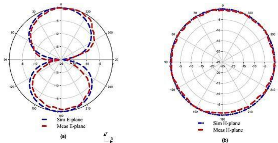
Figure 9. Measured and simulated E-plane and H-plane radiation patterns at 2.4 GHz.
