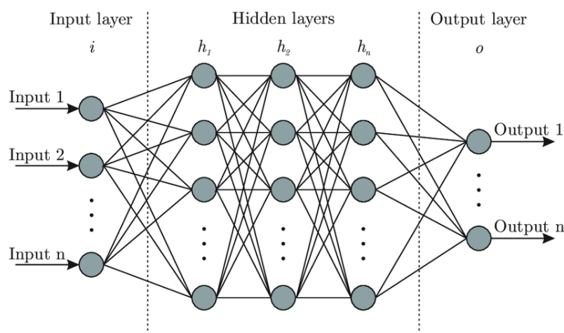
Figure 9 ANN
