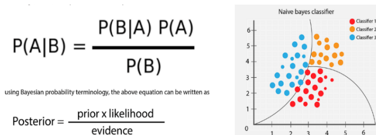
Figure 5 Naïve Bayes
