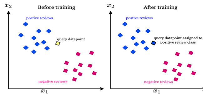
Figure 6 KNN
