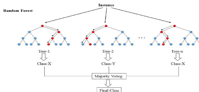
Figure 8 Random Forest
