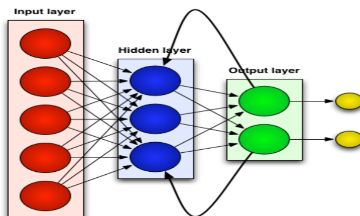
Figure 10. RNN
