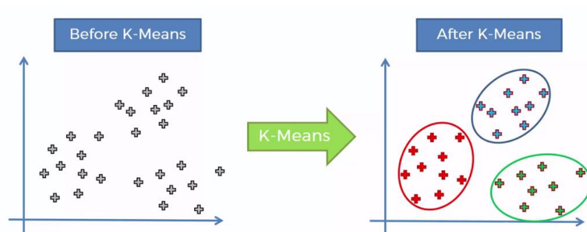
Figure 7 K-Means
