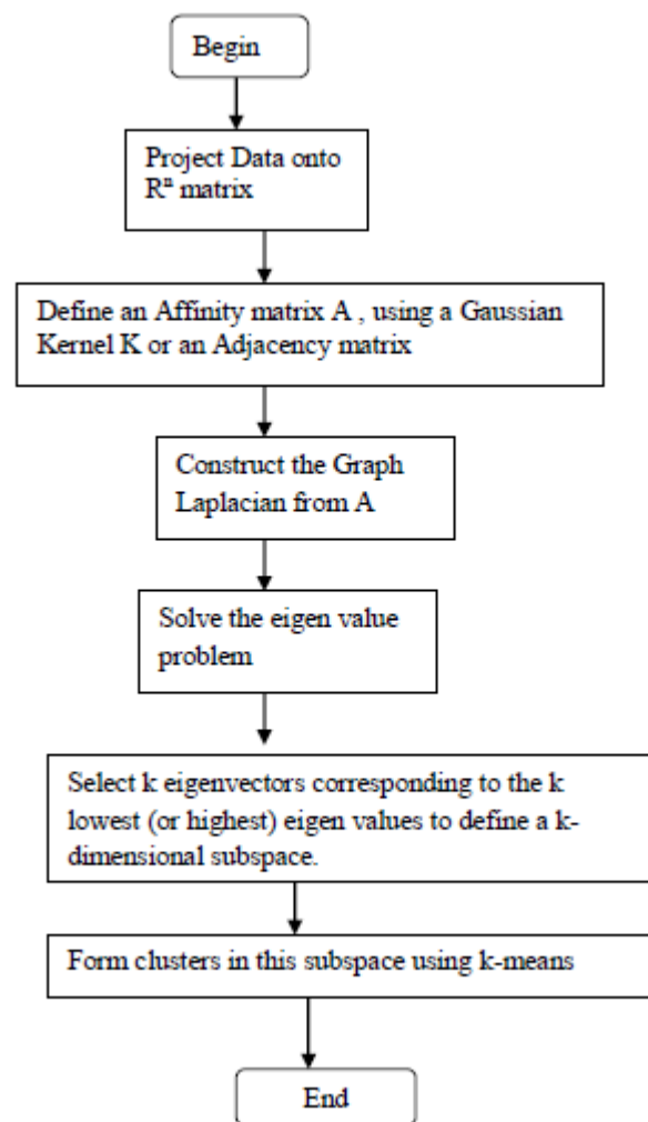
Fig 1: Flowchart of Spectral Clustering
