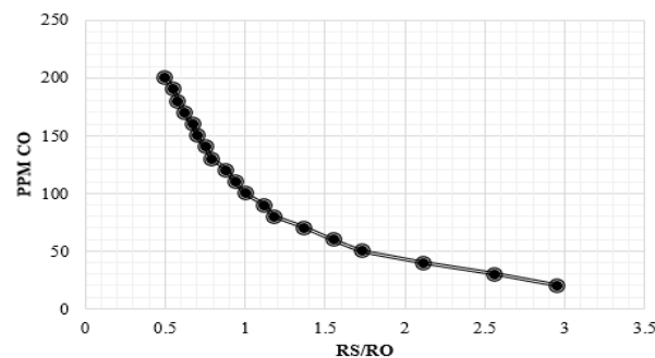
Figure 5. The correlation between PPM CO and Rs/Ro
