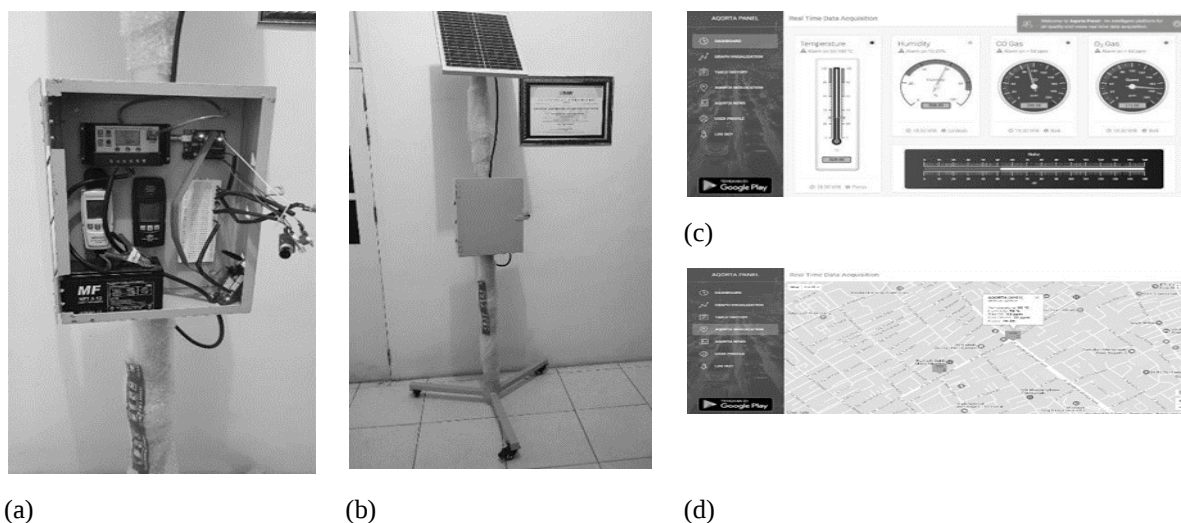
Figure6.(a) Insidetelemetrydevicecasing;(b)Thewholetelemetrydevice;(c)Datareadingofthetelemetrysystem;(d)Locationsoftheinstalledtelemetrydevices
