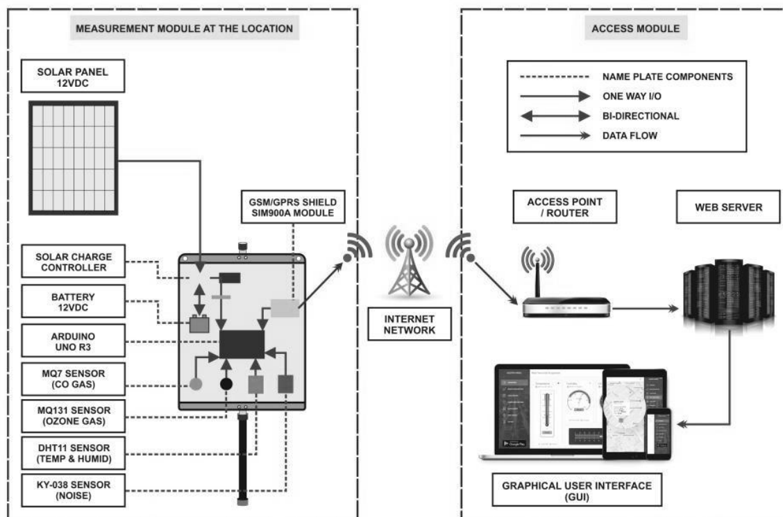
Figure 1. The schematic diagram of real-time air quality and noise monitoring
