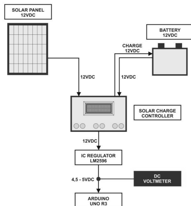
Figure 2. The circuit of solar power system
