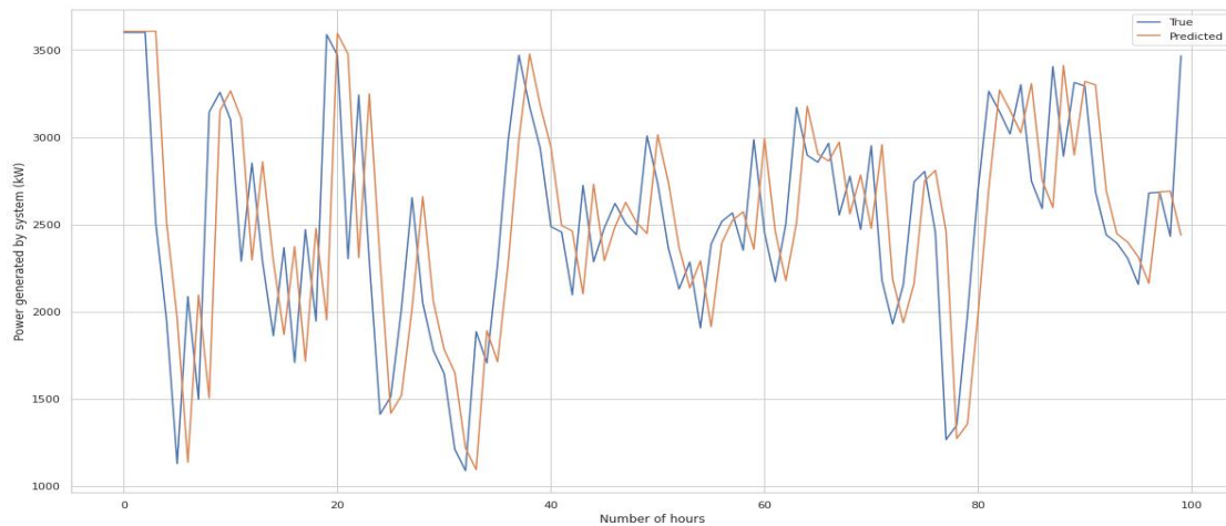
Fig 8: True values and Predicted values of LSTM
