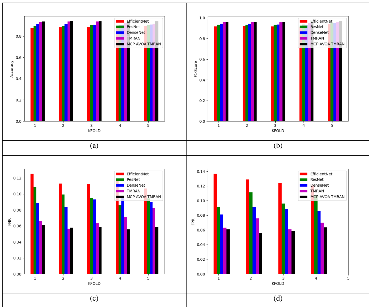
Fig. 5. K-fold validation on recommended Brain Tumor Detection and Severity Classification Model using deep networks among various classifiers in respect to “(a) Accuracy (b) F1-score (c) FNR and (d) FPR.”
