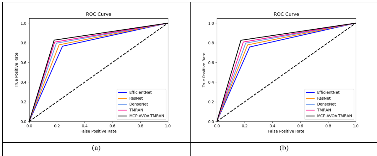
Fig. 9. ROC validation on recommended Brain Tumor Classification Model using deep networks among various optimization algorithms (a) Abnormal classification and (b) Severity classification
