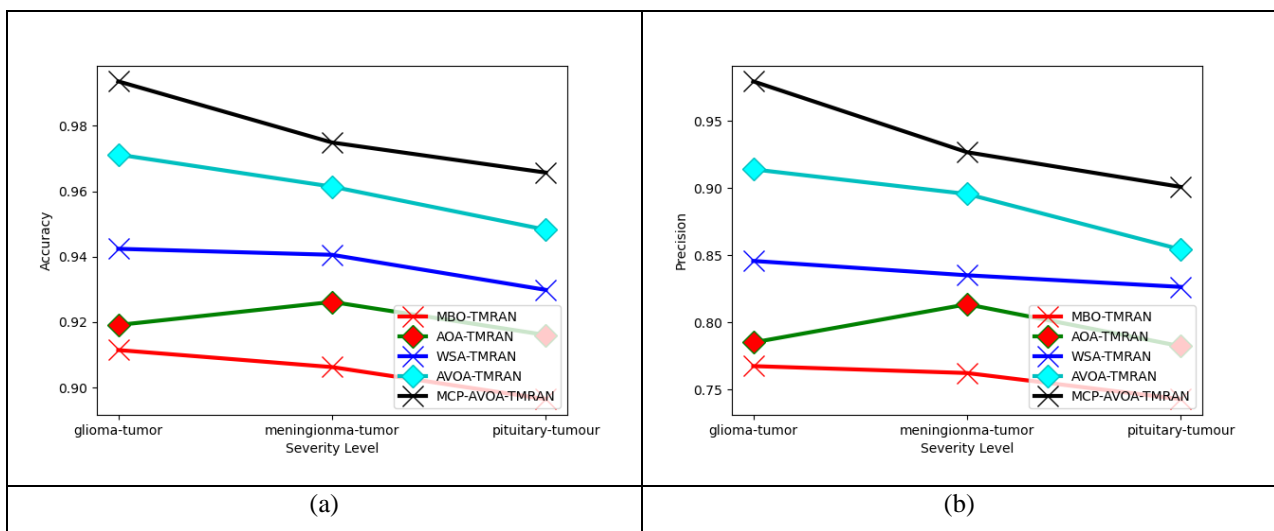
Fig. 6. Severity analysis on recommended Brain Tumor Detection and Severity Classification Model using deep networks among various classifiers in respect to (a) Accuracy (b) Precision (c) Sensitivity and (d) Specificity
