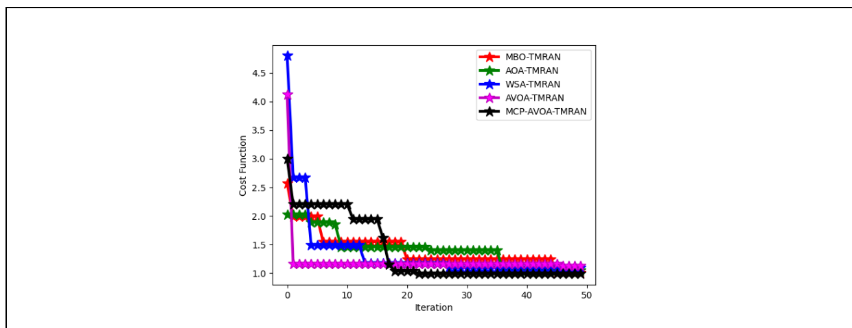
Fig. 8. Cost function validation on recommended Brain Tumor Detection and Severity Classification Model using deep networks among various optimization algorithms
