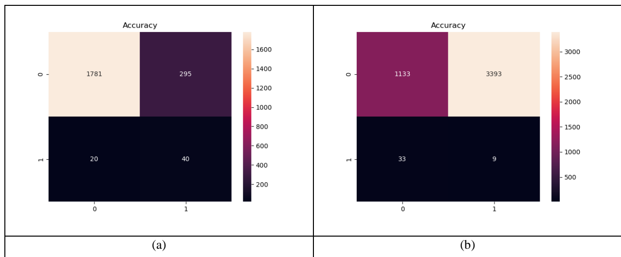
Fig. 10. Confusion Matrix validation on recommended Brain Tumor Detection and Severity Classification Model using deep networks among various optimization algorithms (a) Abnormal classification and (b) Severity classification
