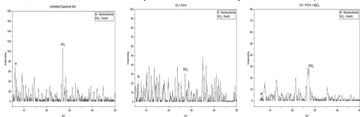
Fig. 5.3 XRD Analysis of Untreated ES, POFA Treated ES, ES+POFA+MgCl 2
