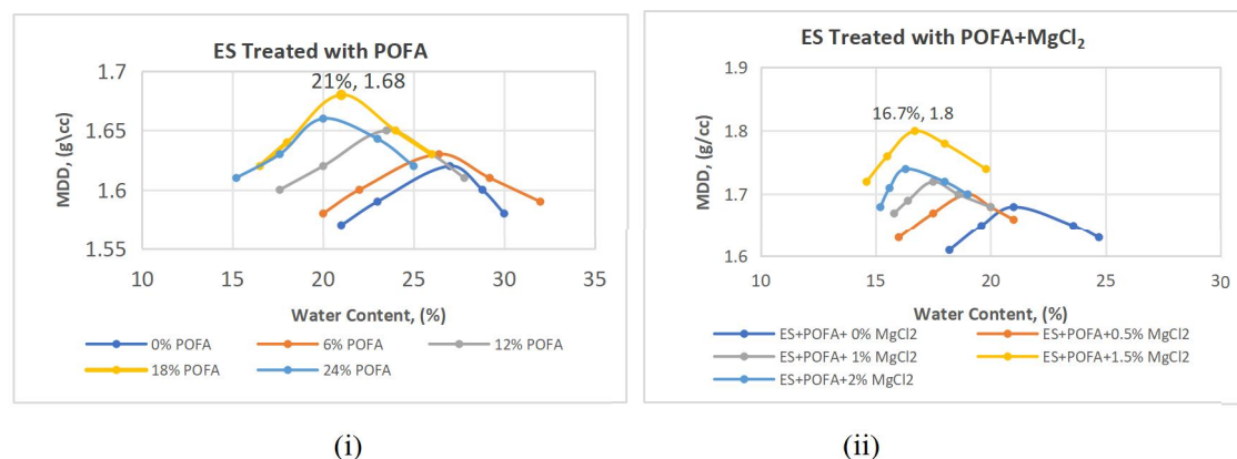
Fig. 5.1: (i) Moisture and Density variation of ES treated with varying percentages of POFA & (ii) ES treated with optimum POFA & various percentages of Magnesium Chloride
