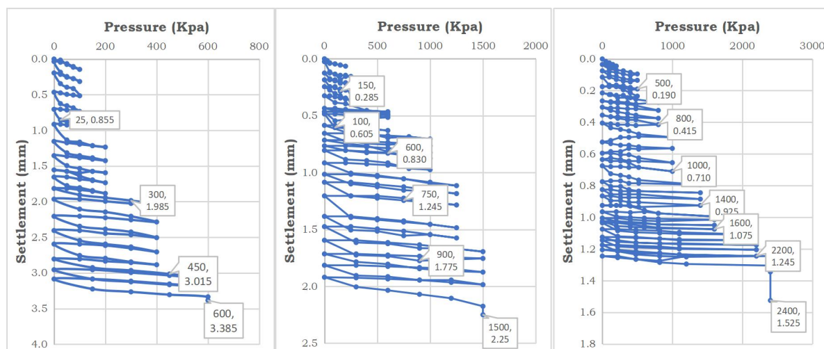
Fig. 5.4 Laboratory CPLT results of Untreated ES, POFA treated ES, Combination of POFA Treated ES+ \text{MgCl}_2
