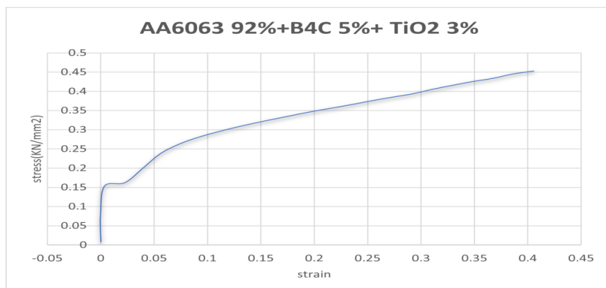
SPECIMEN-9[AA6063-92%,B 4 C-5%,TiO 2 -3%],LOAD-500(GRAM),TIME-100 SECONDS
