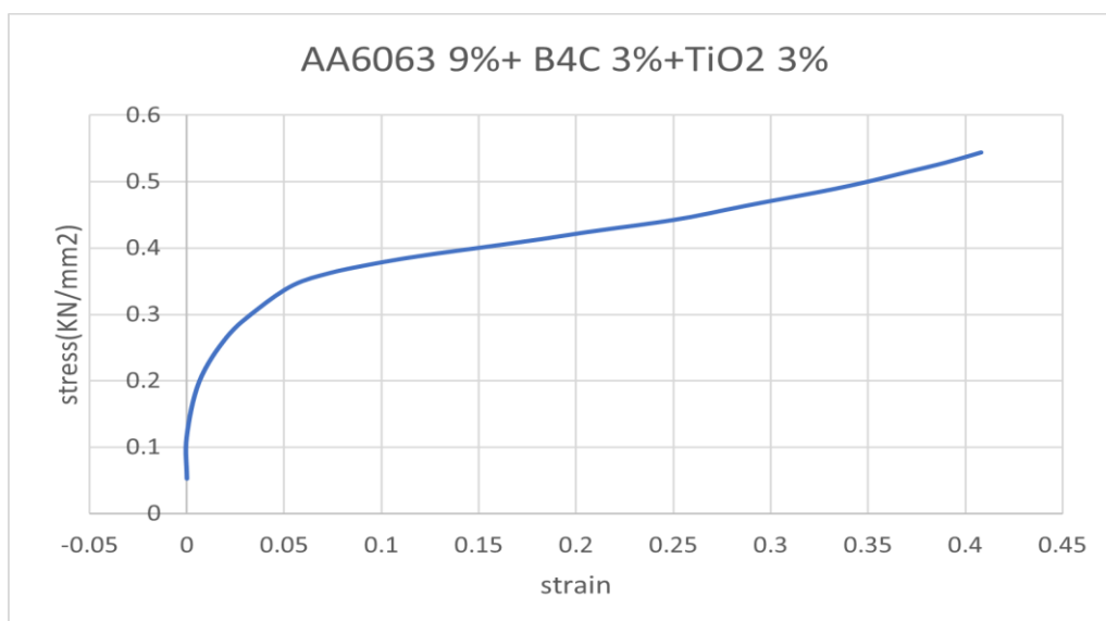
SPECIMEN-6 [AA6063-94%,B 4 C-3%,TiO 2 -3%],LOAD-500(GRAM),TIME-10 SECONDS
