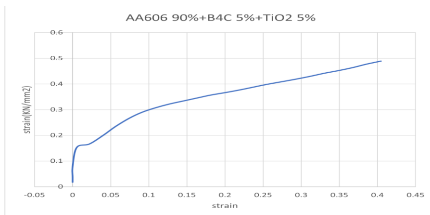
SPECIMEN-10[AA6063-90%,B 4 C-5%,TiO 2 ],LOAD-500(GRAM),TIME-10 SECONDS
