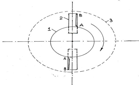
Fig. 1. Diagram of the working chamber of the grain crushing plant by the cutting and impact method: 1-disc; 2-blade; 3- iron mesh.
