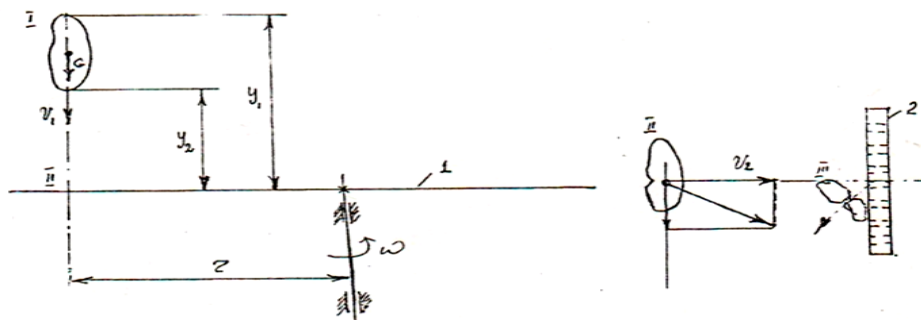
Fig.2. Technological scheme of grain crushing in a rotating crushing chamber operating by the method of free cutting - impact: 1- blade; 2- iron mesh.
