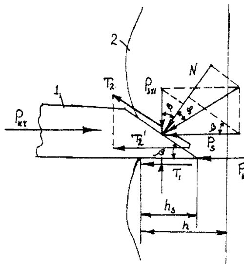
Fig. 3. Forces acting on the knife blade during grain cutting: 1 – knife blade; 2 – grain.
